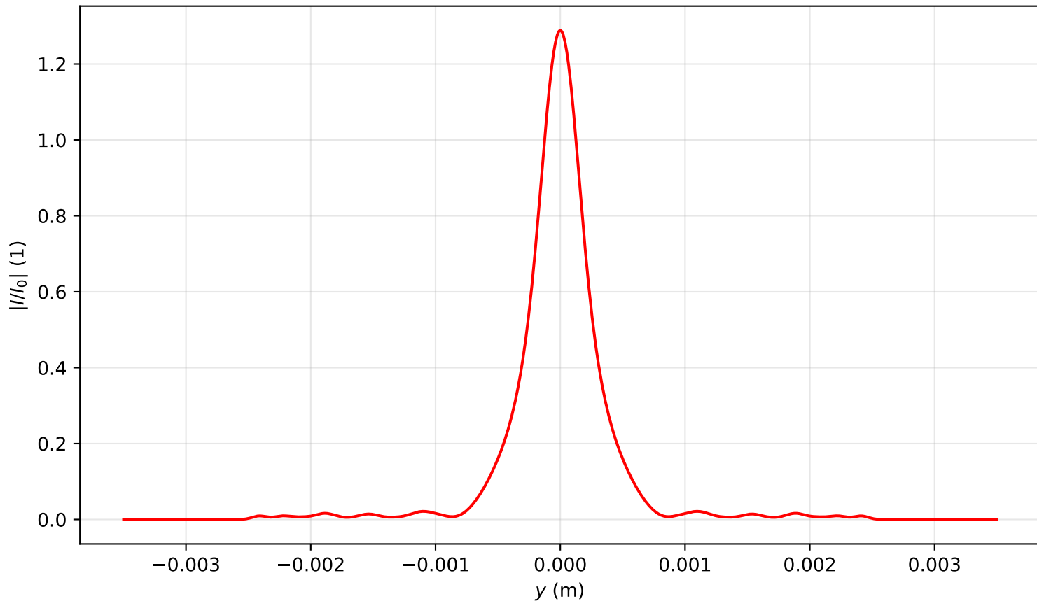
Intensity profile I(x=0, y, z=2.866)/I_0 , P_{in}=2.5P_{cr} , artificial time
